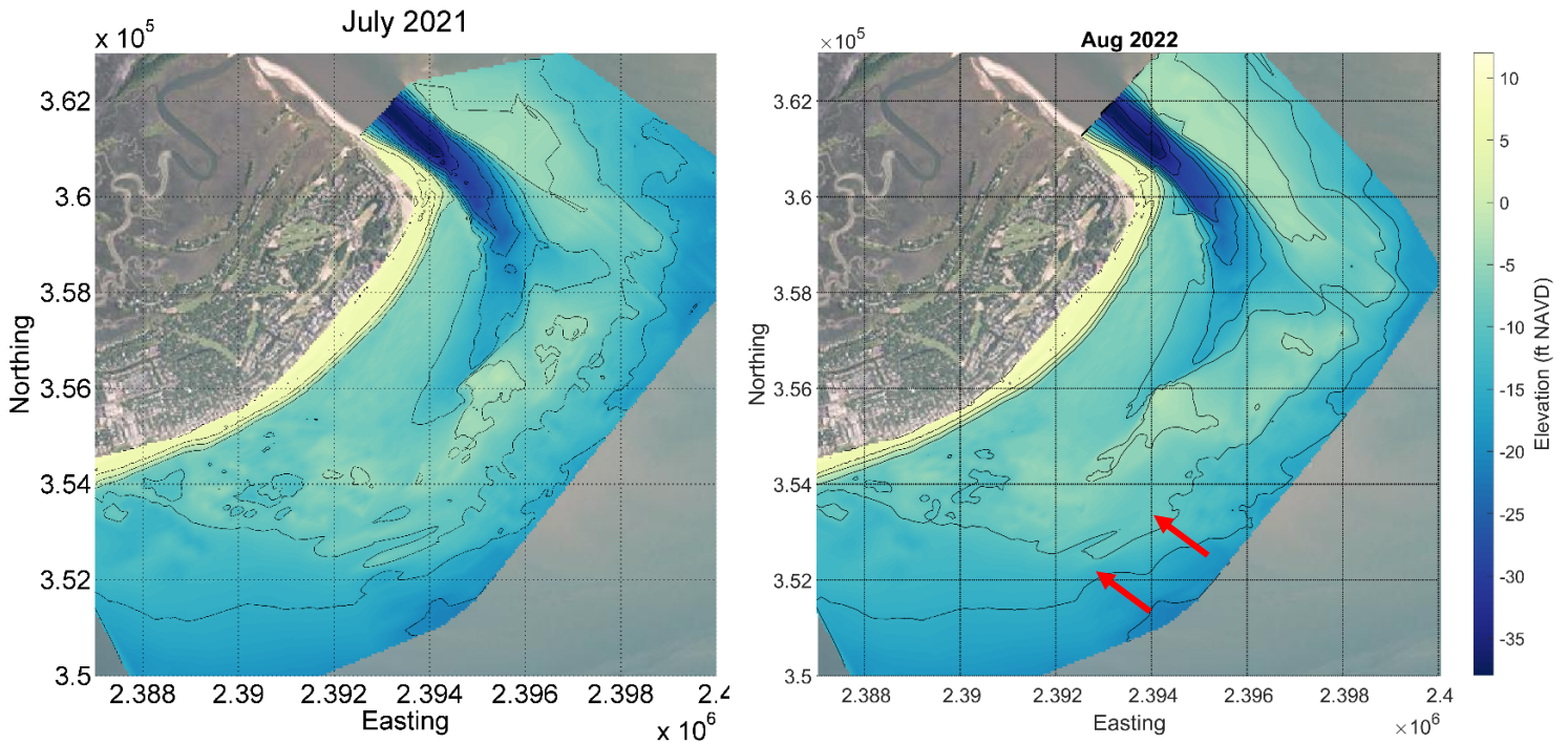
FIGURE 6.1. 2021 and 2022 models of the Dewees Inlet Delta. The most significant change over the past year was growth and onshore migration of a shoal offshore of Beach Club Villas II – Mariners Walk. This shoal will continue to migrate towards the beach, likely attaching in 2-3 years.
