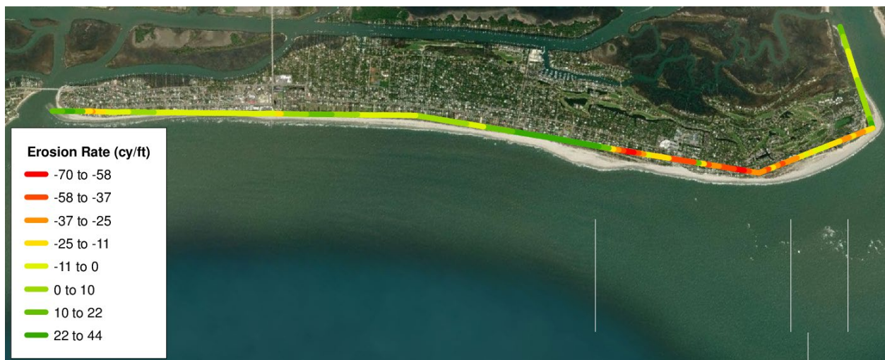
FIGURE 4.1. Line map showing erosion and accretion patterns over Isle of Palms from July 2021 – Aug 2022.
