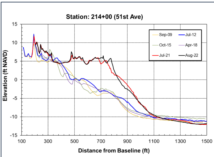
FIGURE 4.19. [LEFT] Profiles along Reach 4 show accretion has led to gains of over 300 ft of dry sand width and formation of new dune ridges. [RIGHT] Ground photos from Station 170 [UPPER], Station 200 [MIDDLE], and Station 216 [LOWER] in August 2022.
