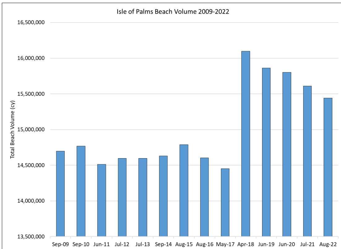
FIGURE 4.3. Total beach volume at Isle of Palms from 2009 to 2022. Effects of the 2018 project are seen in the rapid increase in the April 2018 island-wide beach volume.
