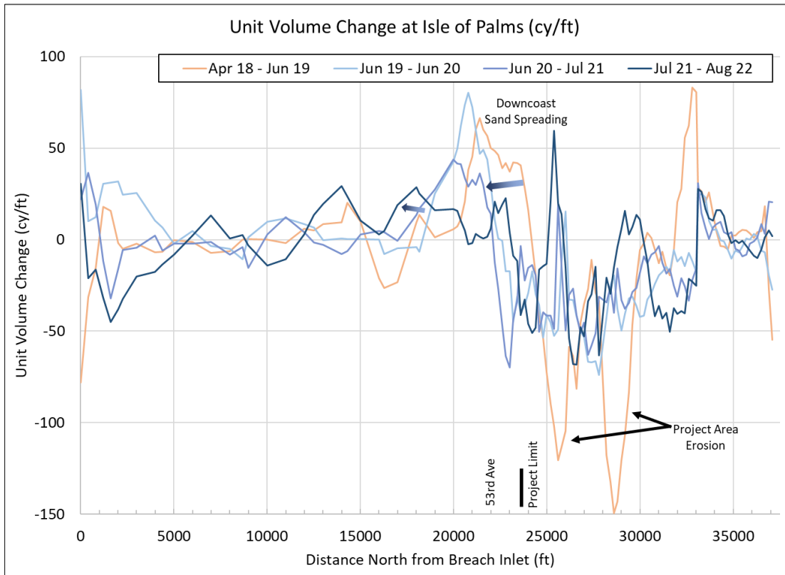
FIGURE 4.2. Beach unit volume change between each monitoring event at Isle of Palms. The X axis represents distance from Breach Inlet. This graph highlights the erosion occurring in the project area and accumulation of spreading sand adjacent to the project area.
