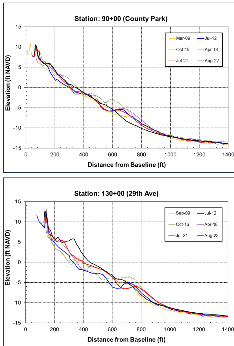
FIGURE 4.22. Example profiles from Reach 3. At station 90+00, there was a net loss of volume due to movement of the underwater sandbar. The dry beach remained stable over the past year.
