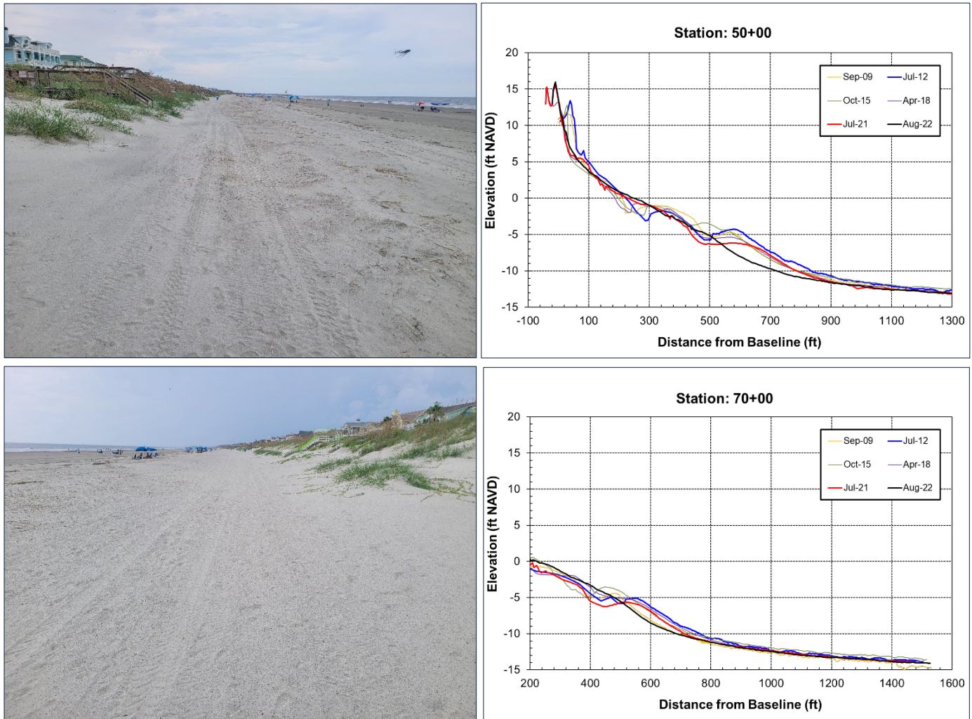
FIGURE 4.25. Aug 2022 photos of Reach 2. [UPPER LEFT] View north from Station 50. [LOWER LEFT] View west from Station 70. The photos show a healthy beach with dry sand seaward of the dune. Profiles show that the dune remains more landward than the 2012 condition; however, it has been fairly stable since 2017.
