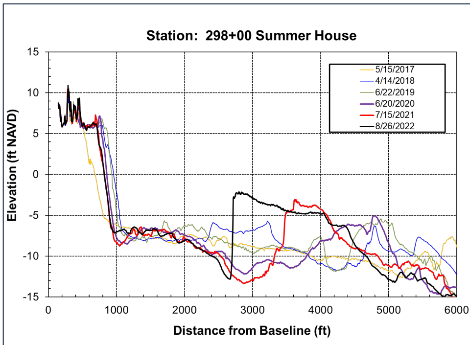
FIGURE 6.2. Profiles from stations 282 [UPPER] and 298 [LOWER] showing growth and onshore migration of a large shoal in Dewees Inlet. At both locations, the shoal moved ~750 landward over the past year. The shoal is exposed at low tide off of Summer House.
