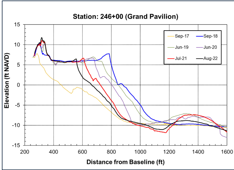
FIGURE 4.13. Reach 5 profiles.
